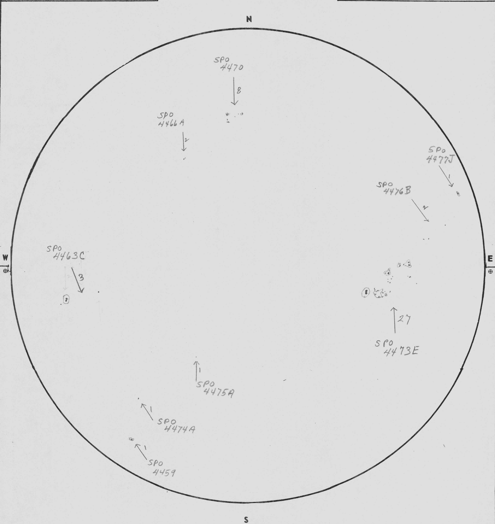
SACRAMENTO PEAK OBSERVATORY SUNSPOT, NEW MEXICO
