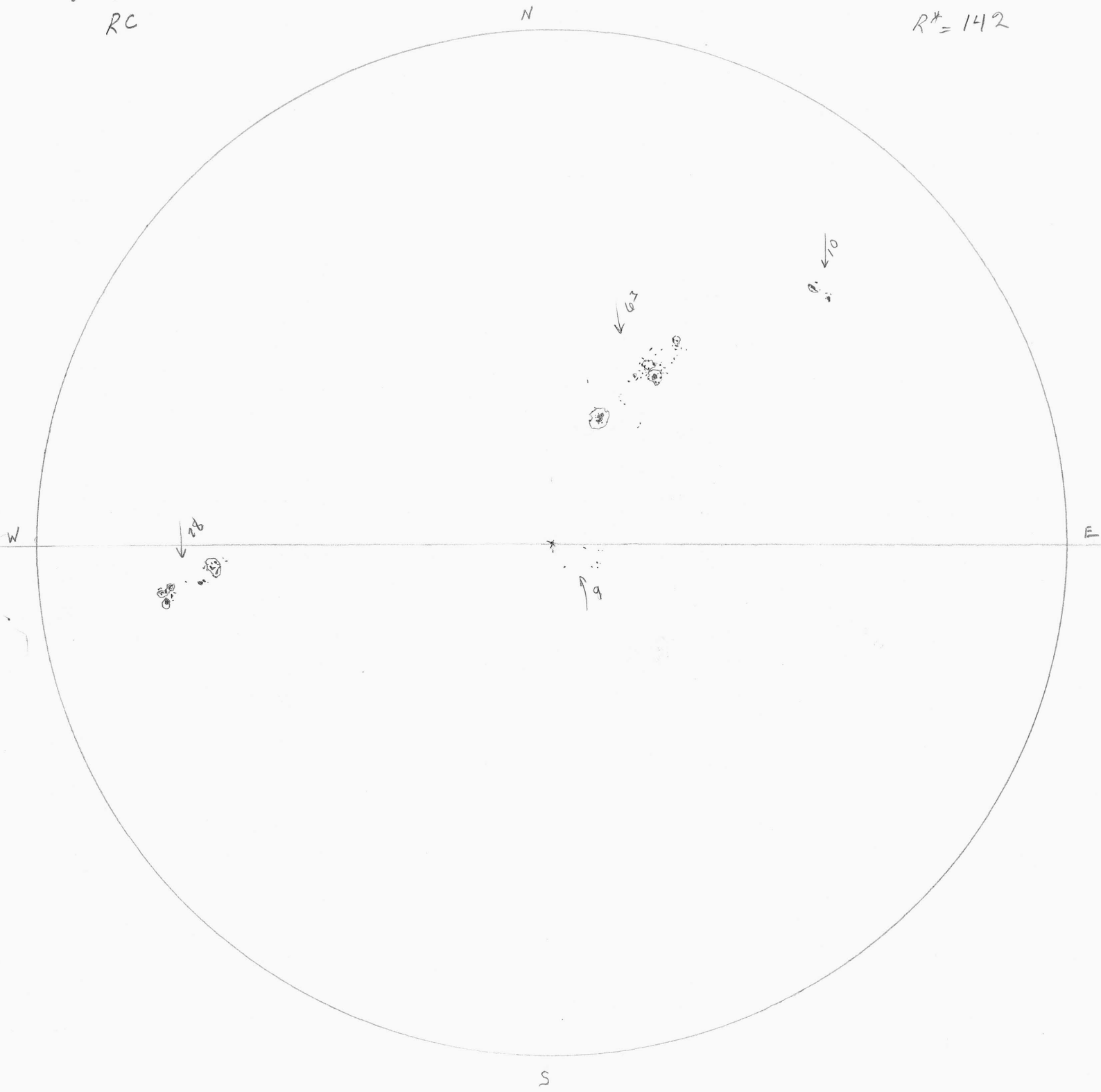
SUNSPOT DRAWING
