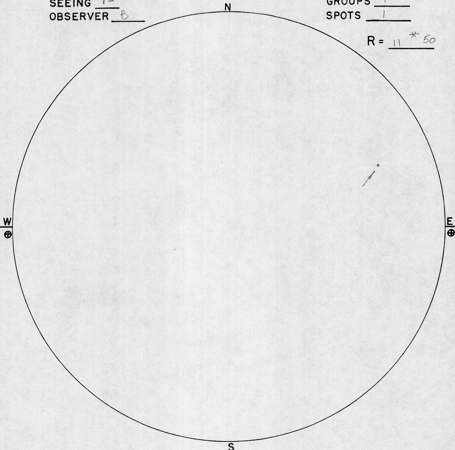
S SUNSPOT DRAWING SACRAMENTO PEAK OBSERVATORY SUNSPOT, NEW MEXICO
