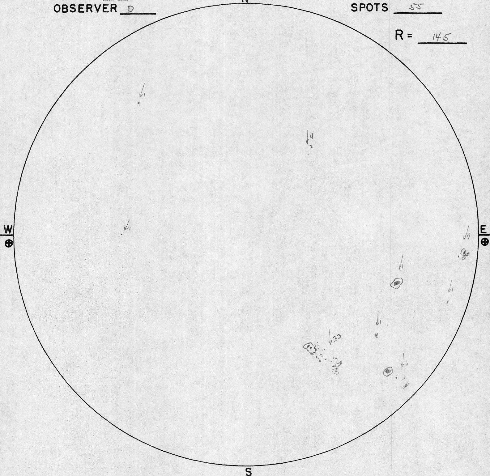
S SUNSPOT DRAWING SACRAMENTO PEAK OBSERVATORY SUNSPOT, NEW MEXICO
