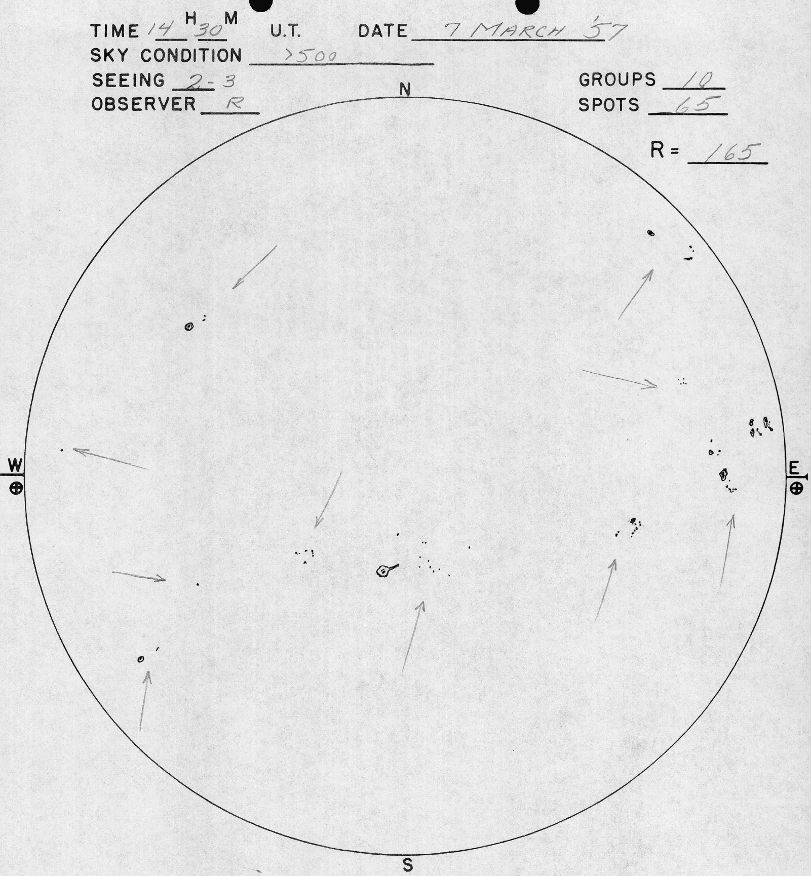
SUNSPOT DRAWING SACRAMENTO PEAK OBSERVATORY SUNSPOT, NEW MEXICO
