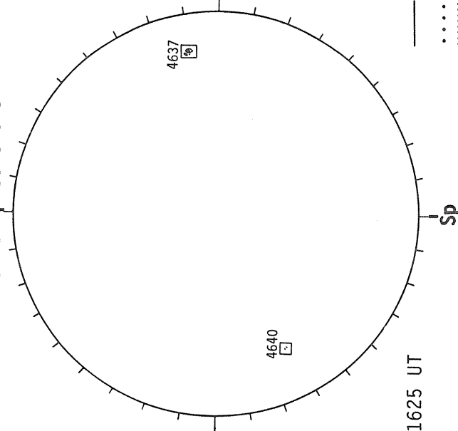
HOLLOMAN SUNSPOTS
