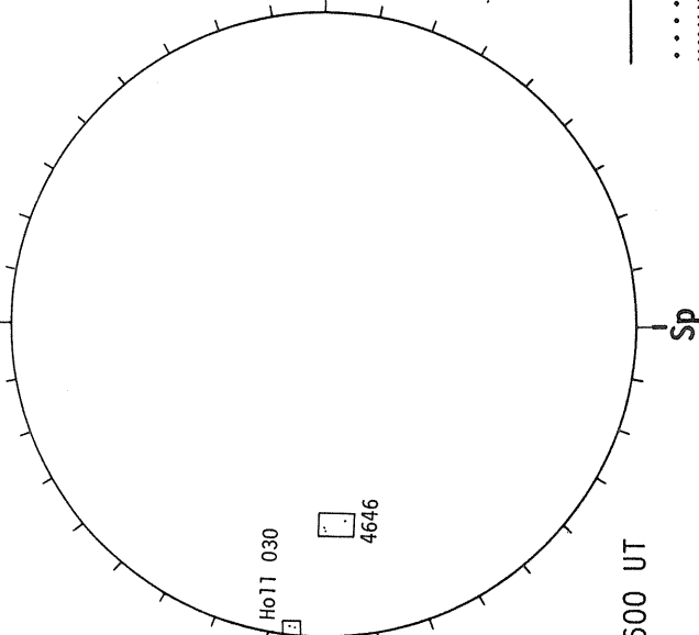
HOLLOWAY SUNSPOTS
