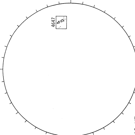
HOLLOMAN SUNSPOTS
