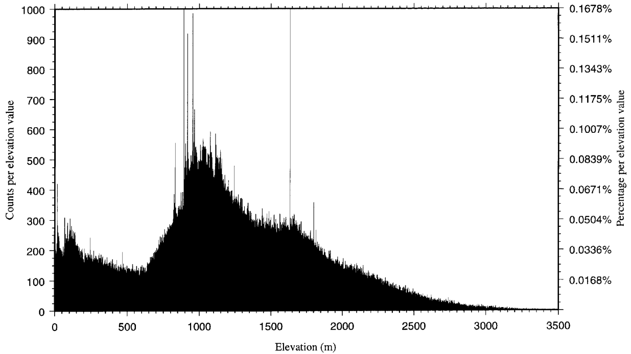
Plate 9. Blend of DTED Breakline and Median DEMs: Parts of Turkey (linear plot)
