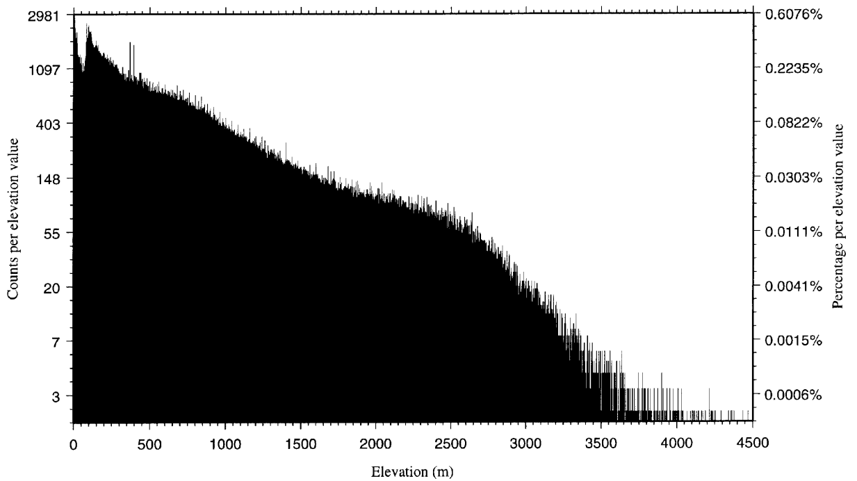
Plate 17. SGN/NGDC DEM: Italy (semi-logarithmic plot)
