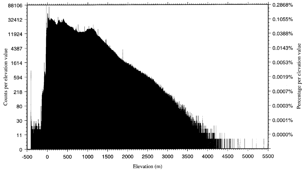
Plate 2. DTED Discrete DEM: Parts of Africa and Europe (semi-logarithmic plot)
