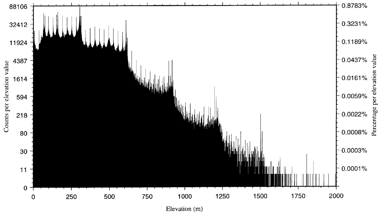
Plate 13. DCW-based DEM: Australia (semi-logarithmic plot)
