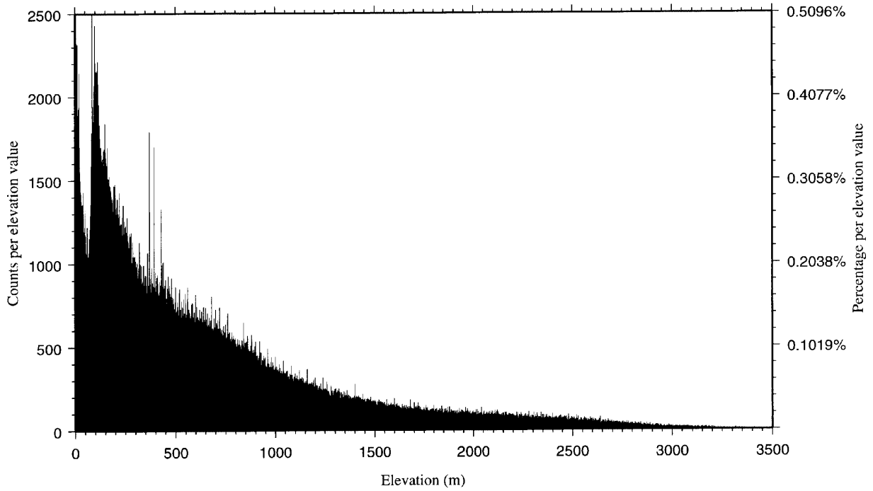
Plate 16. SGN/NGDC DEM: Italy (linear plot)
