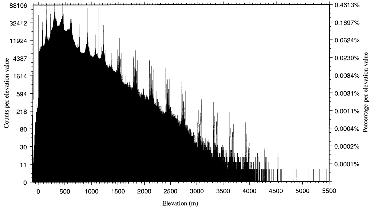
Plate 22. DCW-based DEM: Parts of Africa and Europe (semi-logarithmic plot)
