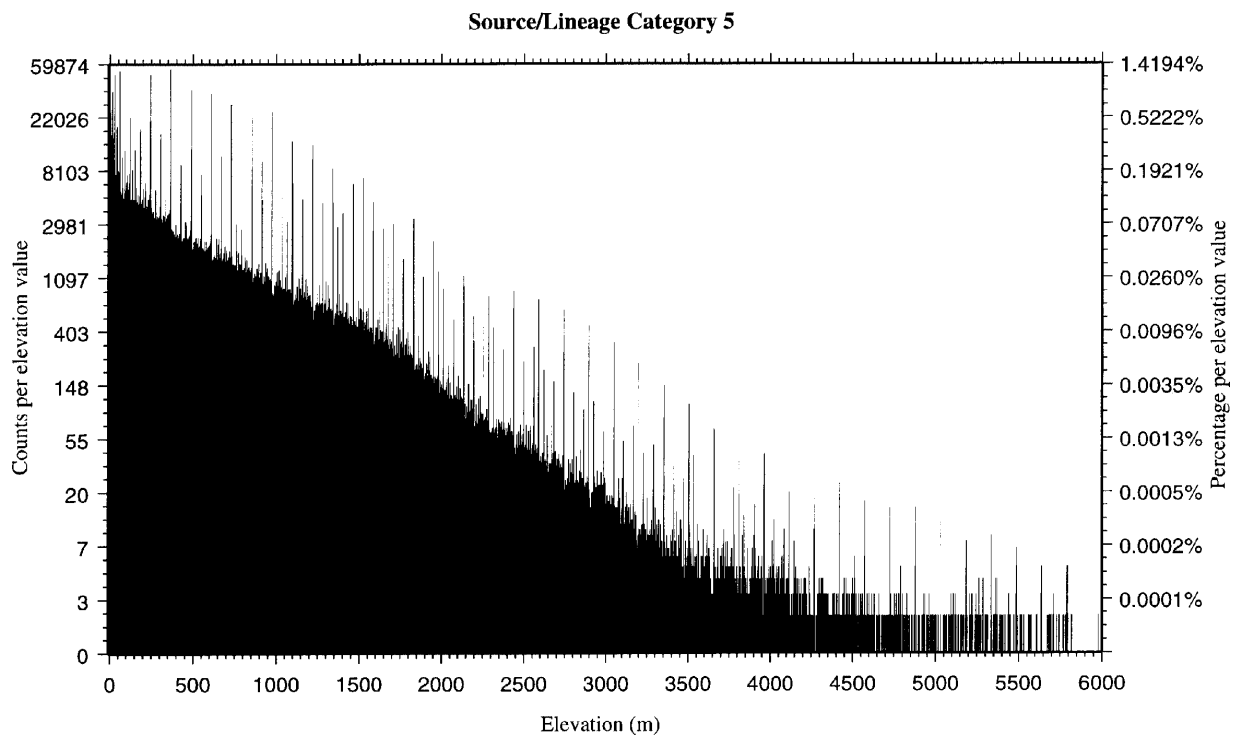
Plate 11. DMA/USGS DEM: Parts of North America (semi-logarithmic plot)
