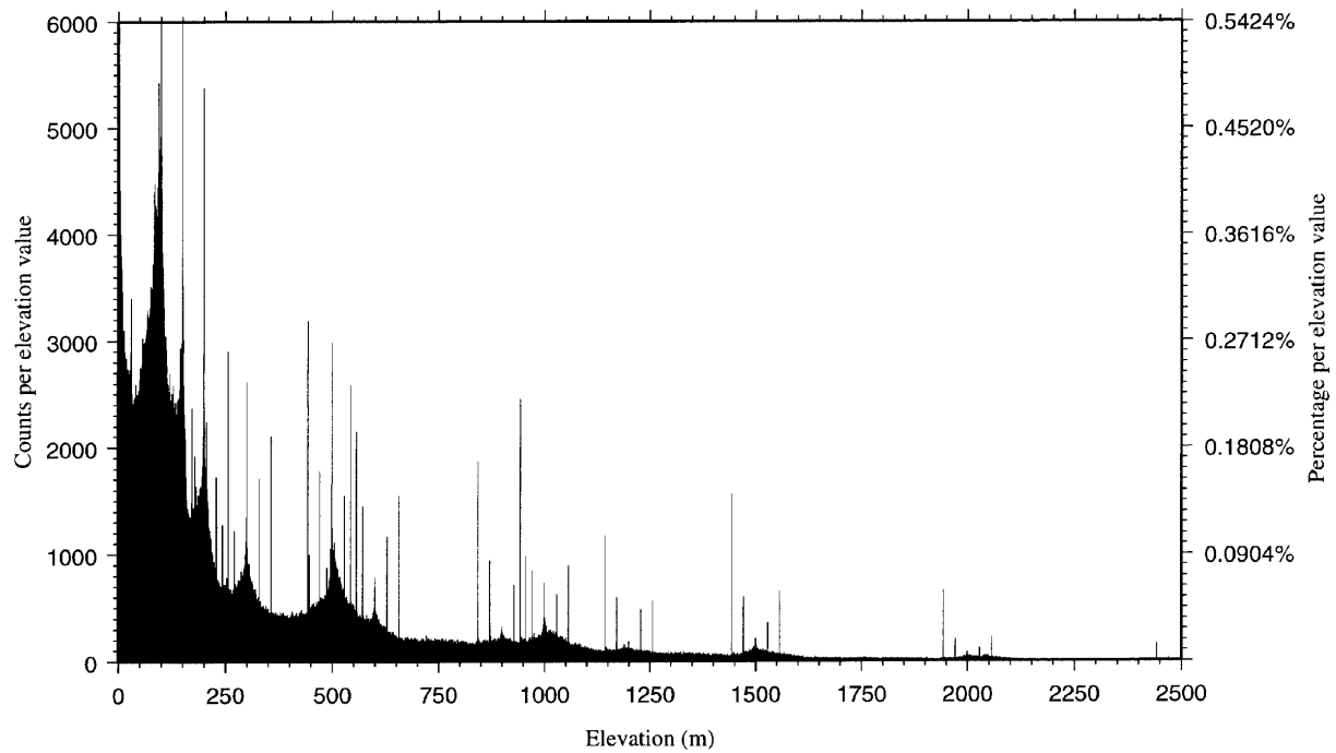
Plate 27. DEM Derived from AMS Maps: Parts of Southeast Asia (linear plot)
