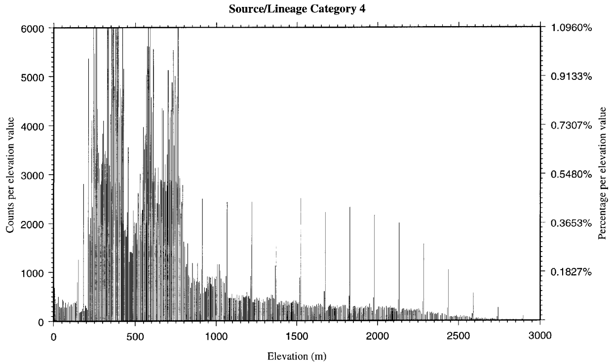
Plate 10. DTED/NGDC DEM: Parts of North America (linear plot)
