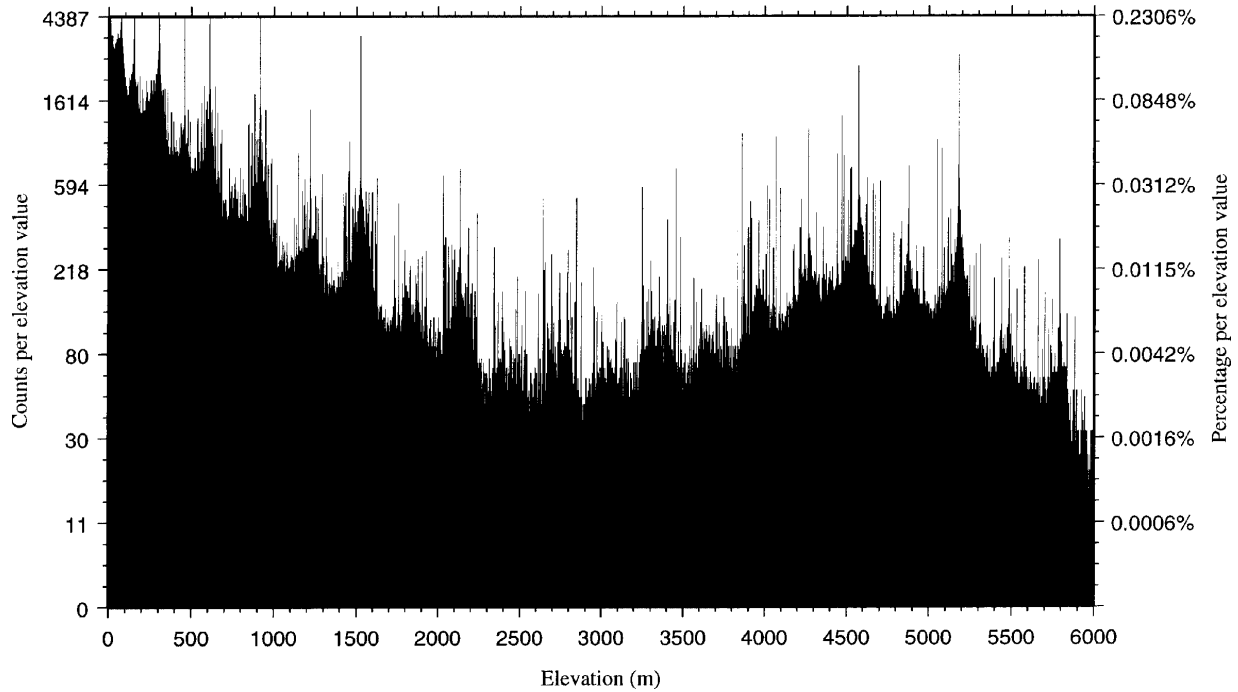
Plate 23. DCW-based DEM: Parts of Asia (semi-logarithmic plot)
