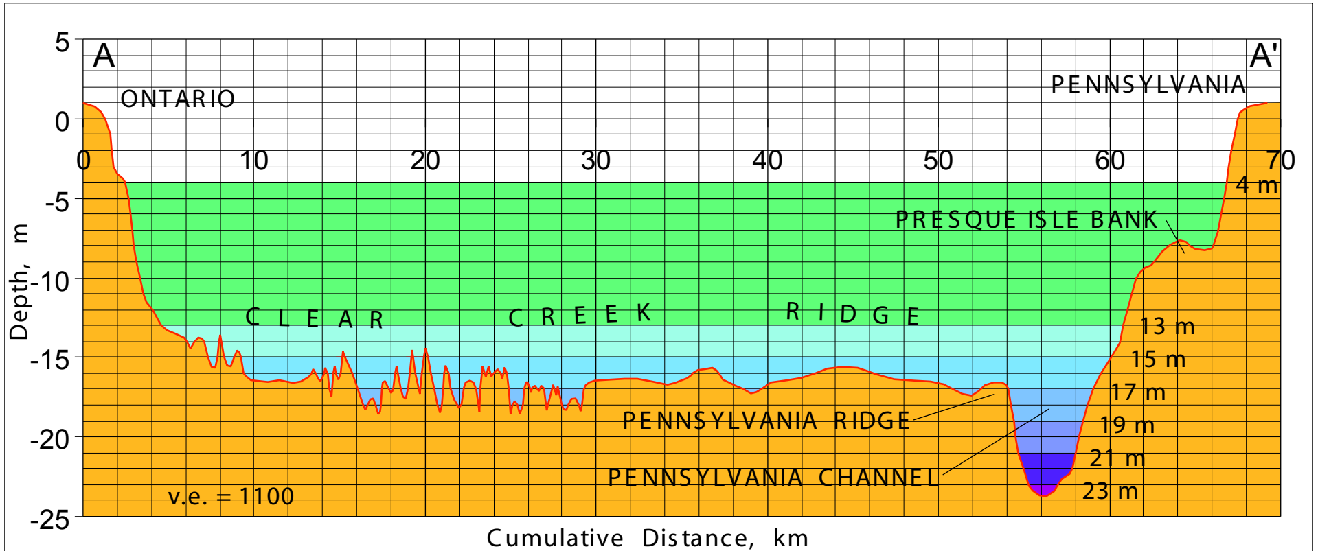
Figure 7 - Longitudinal section along the crest line of Clear Creek Ridge. Color bands depict specific depth intervals and are the same for both sections, figure 7 and figure 8, to facilitate comparison. The 4-meter line is suggestive of lake water depth following the Nipissing Rise in lake level.
