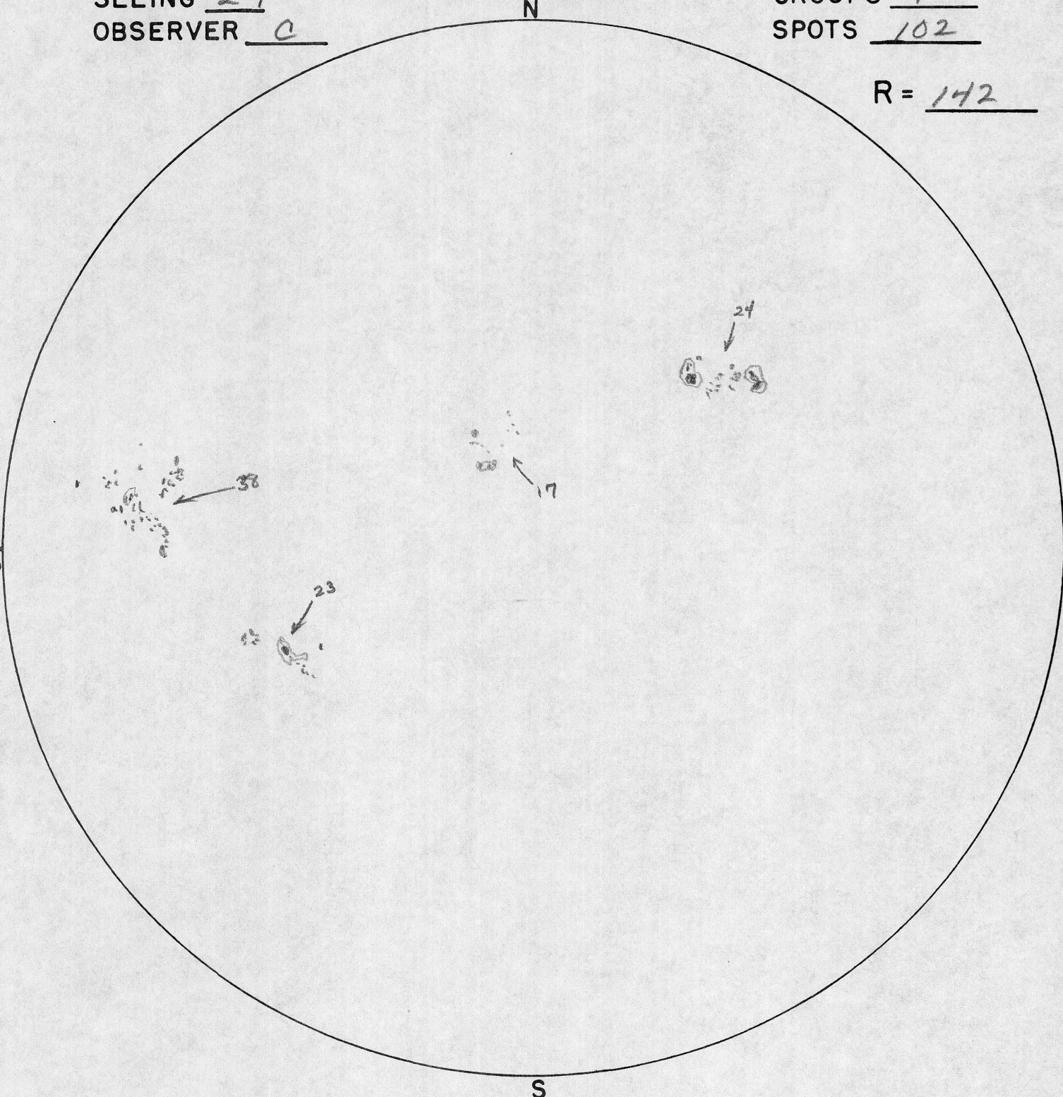
SUNSPOT DRAWING SACRAMENTO PEAK OBSERVATORY SUNSPOT, NEW MEXICO
