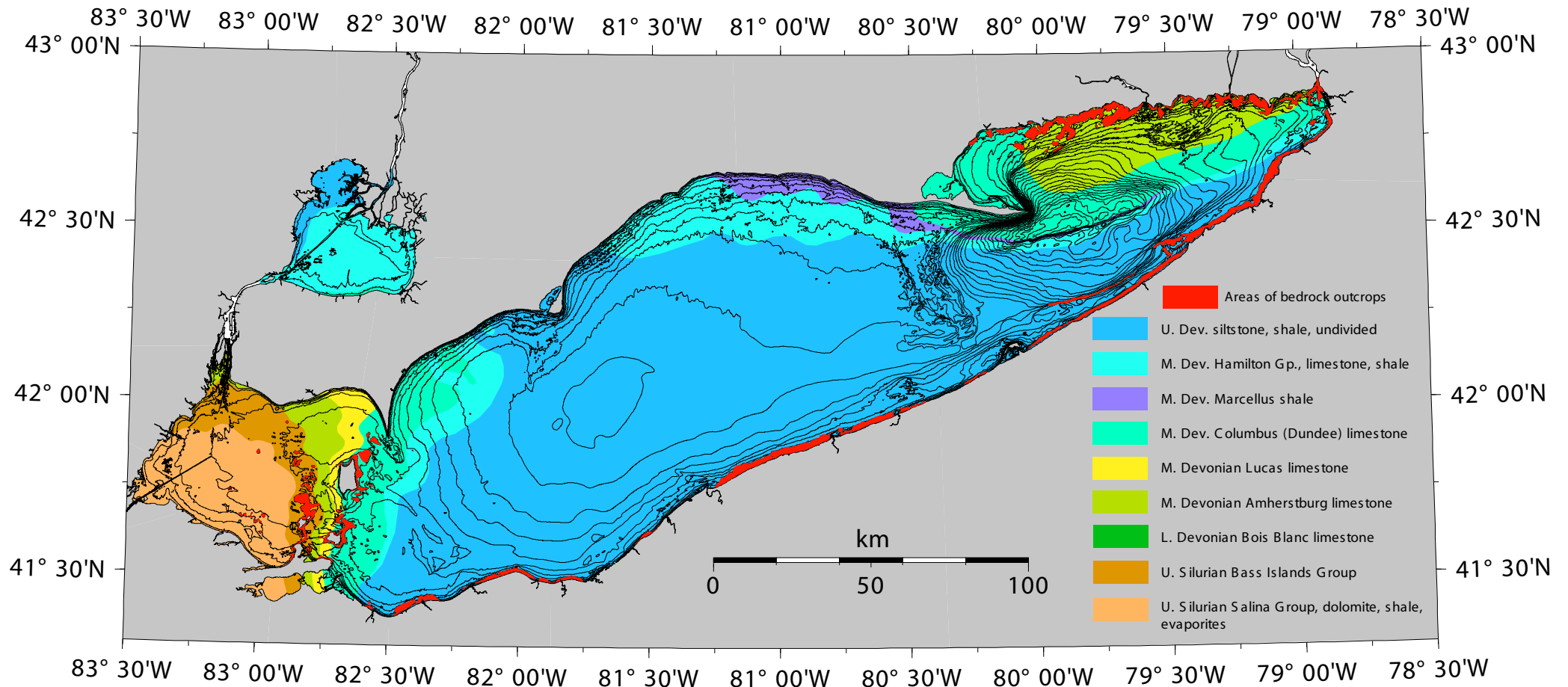
Figure 2 - Areas of bedrock outcrops in Lake Erie. Locations of bedrock outcrops shown here are adapted from compilations by Lewis in Sly and Lewis (1972); Rukavina (1976); Thomas, et al. (1976); and Fuller and Foster (1998); and altered to fit the bathymetry. Bedrock outcrops in Lake Erie occur along the shores of eastern Lake Erie, in several locations along the southern shore of the Central Basin, and in the Islands area. Bedrock geological boundaries beneath the Lake are tentative and are adapted from Sanford and Baer (1971). The ultimate mapping of bedrock geology will require integration of inferred lakefloor geology with onshore geological mapping carried out over an extended period of time by four states and one province - a daunting task not undertaken within the limited confines of this paper.
